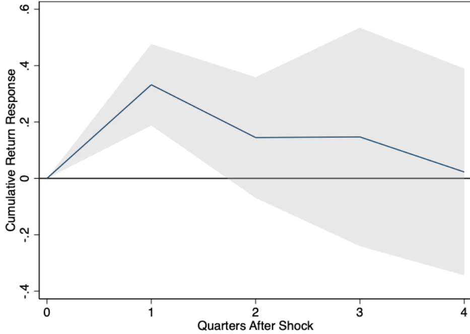
Figure 4: Price Impact Dynamics
