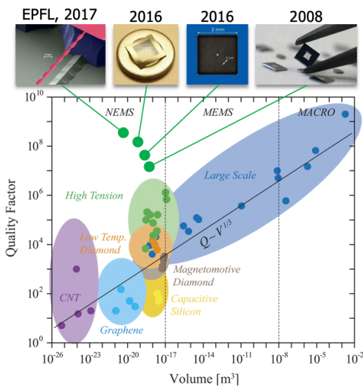
Figure 1 : Strain engineering and soft clamping for ultra coherent mechanical oscillators (figure adapted from Imboden et al.)
