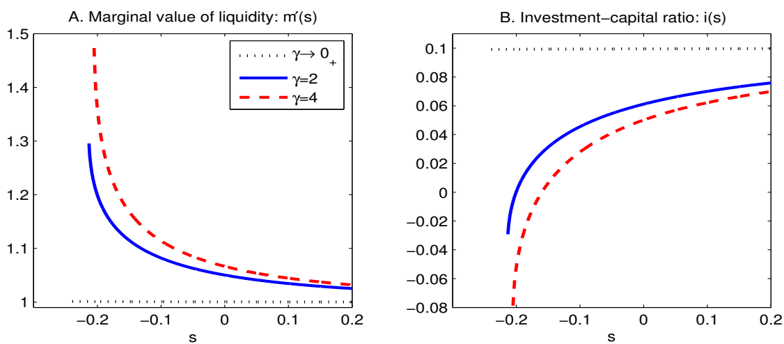
Figure 15: Effects of the entrepreneur's risk aversion. Panels A and B plot the marginal (certainty equivalent) wealth of s , m'(s) , and the investment-capital ratio i(s) , respectively. The dotted, solid, and dashed lines correspond to three different levels of risk-aversion, \gamma \rightarrow 0_+ , \gamma = 2 , and \gamma = 4 , respectively.
